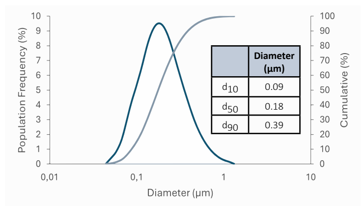
Slurry - 50 wt% - pH 8.5 - PSD (Horiba)
